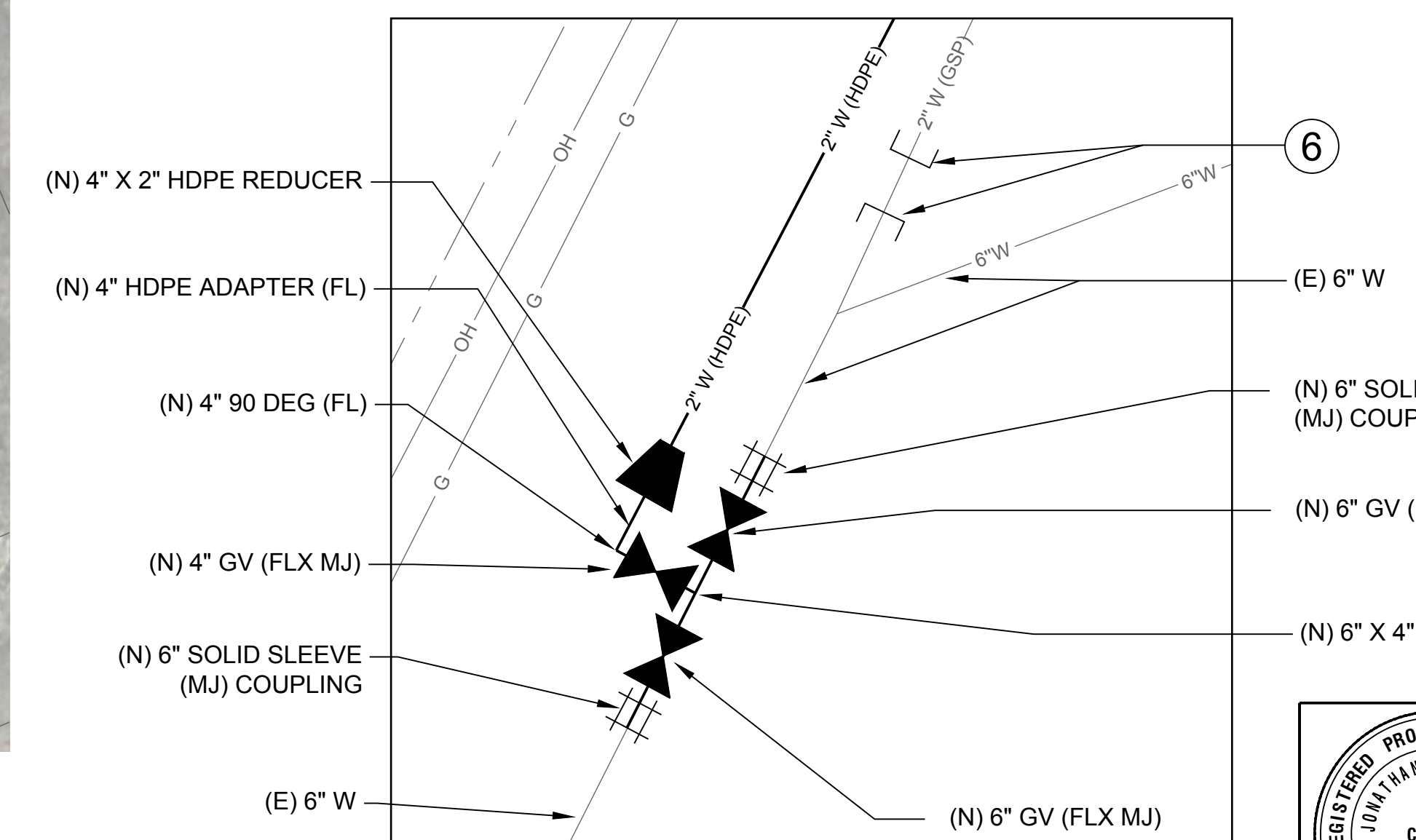
CONNECTION DETAIL
